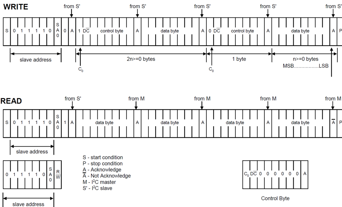
Figure 7 I 2 C Protocol
