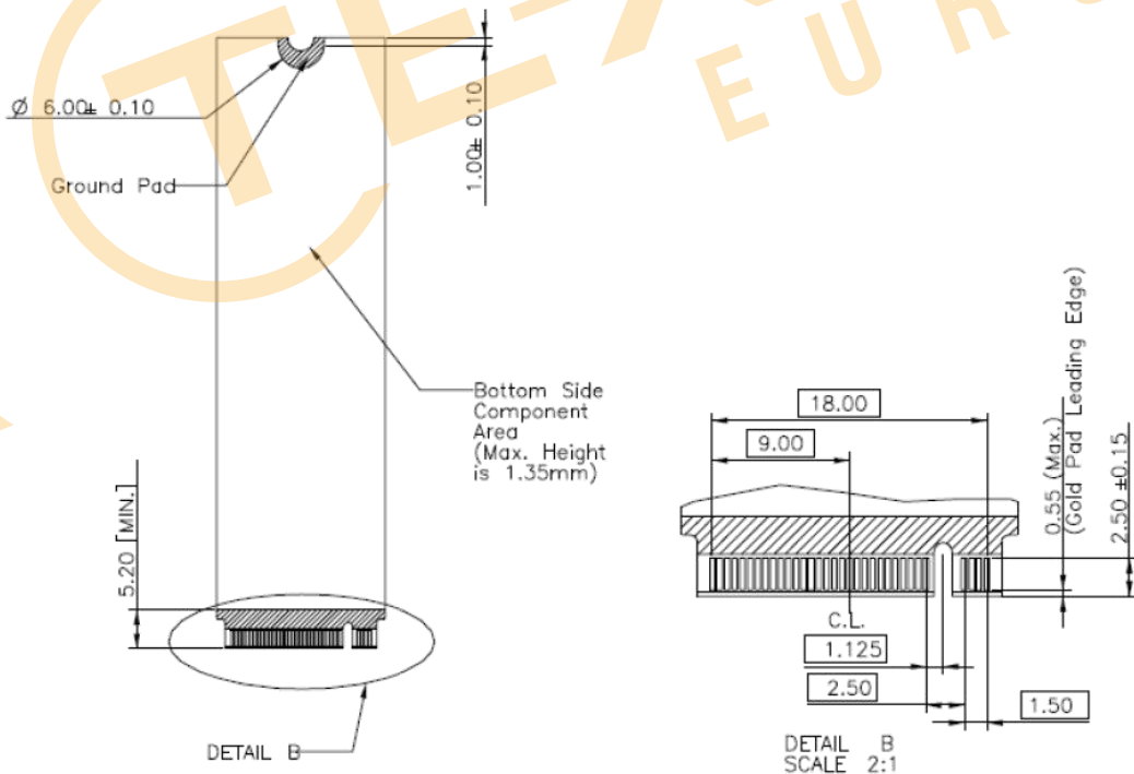
Bottom View
