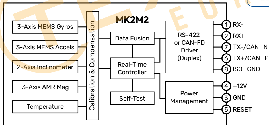
Figure 2: OSCP-MK2M2 Functional Block Diagram
