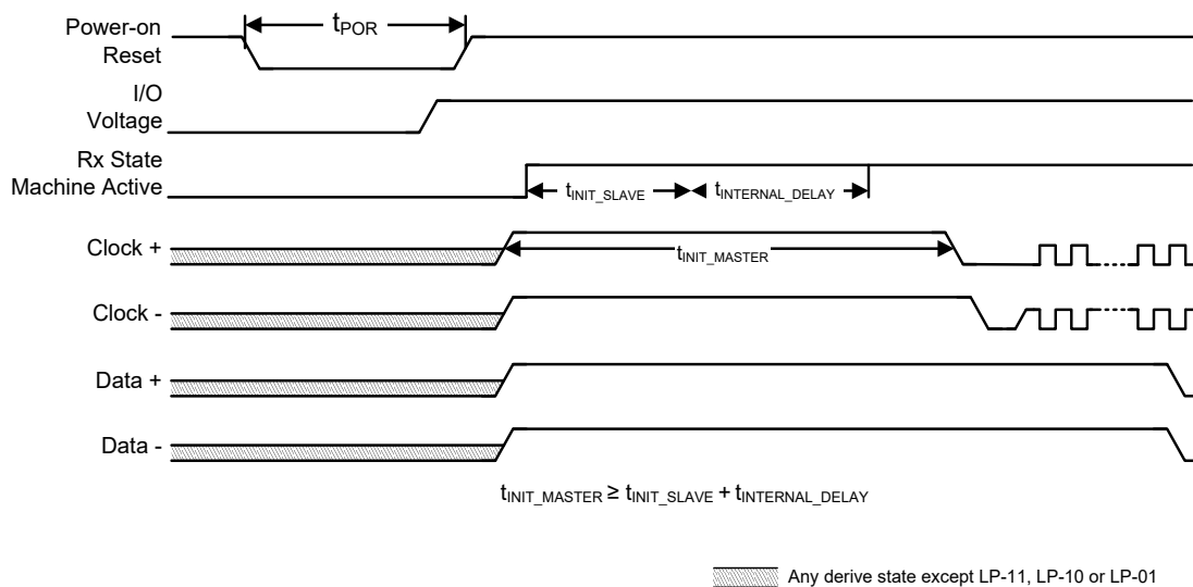
Figure : Peripheral Power-Up Sequencing Example
